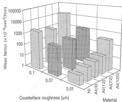
Fig. 4. Wear factor vs. counterface roughness and age of polyethylene.
