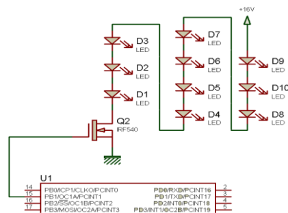
Gambar 4. Rangkaian Driver LED
